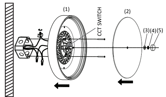
wall mounting.
