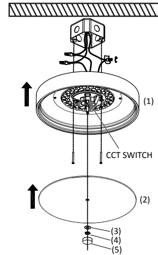
ceiling mounting.
